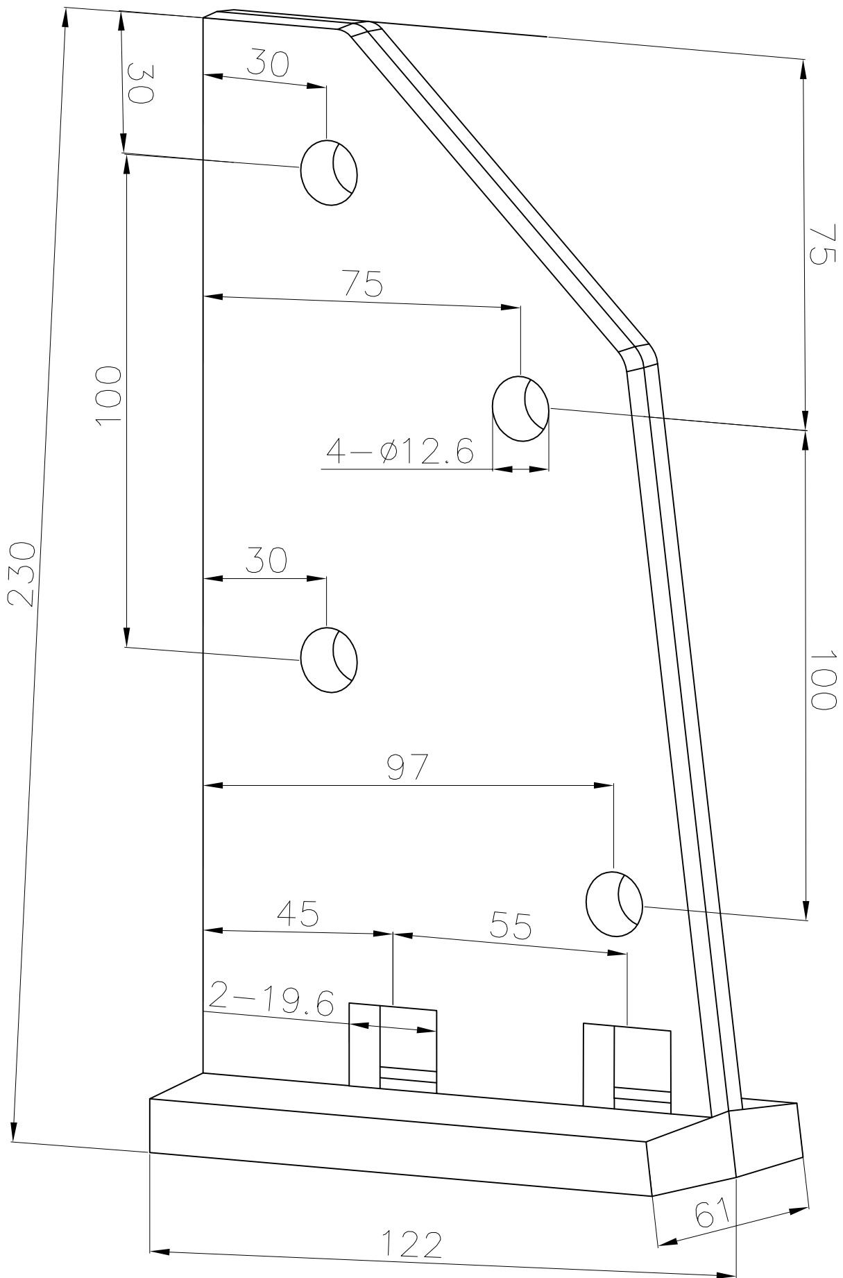
Rafter bracket
